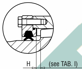
Double-lip seal type TN559
