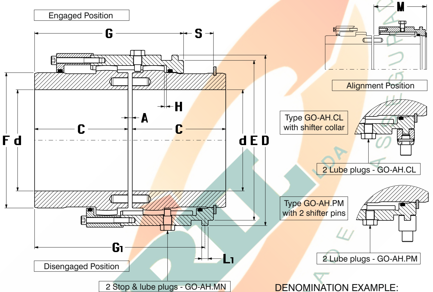
Fig. 28 - GO-AH.MN Coupling
