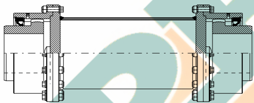
E.g. G35-FS SPACER COUPLING SIZE 60
