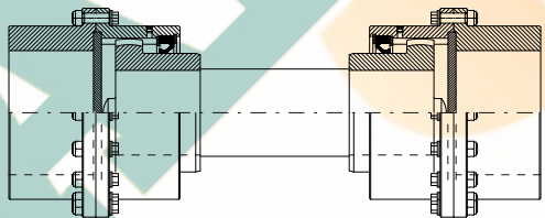
E.g. G35-FR FLOATING SHAFT COUPLING SIZE 60
