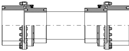
Fig. 56 - AO-FB.HT.C Floating Shaft Coupling
