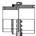
AO-FB.D & AO-FB.HT.D Floating Shaft Couplings
