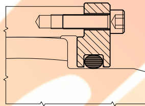
Removable side flanges design, available on demand for sizes from 4 to 11 denomination example GO-6A.C
