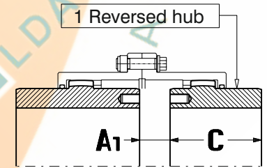
Fig. 07 - GO-AMR Coupling
