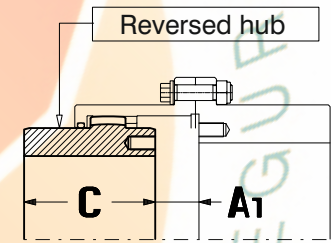
Fig. 09 - GO-FAR Coupling
