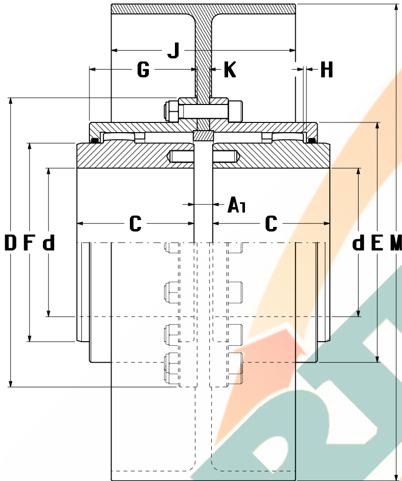
Fig. 23 - GO-A.FF Coupling
